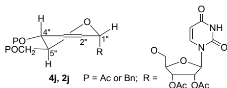
Figure 1. Preferred conformations of compounds 4j and 2j .
